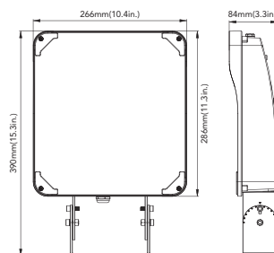
90W&120W(Yoke Mount)
