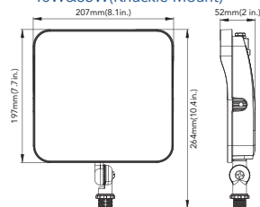
40W&65W(Knuckle Mount)
