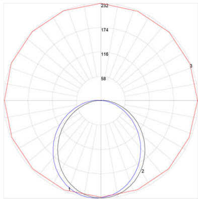
Maximum Candela = 232.14 Located At Horizontal Angle = 157.5, Vertical Angle = 4 # 1 - Vertical Plane Through Horizontal Angles (157.5 - 337.5) (Through Max. Cd.) # 2 - Vertical Plane Through Horizontal Angles (0 - 180) # 3 - Horizontal Cone Through Vertical Angle (4) (Through Max. Cd.)
