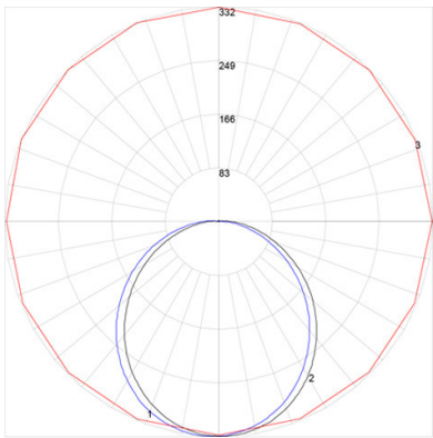
Maximum Candela = 331.95 Located At Horizontal Angle = 112.5, Vertical Angle = 3 # 1 - Vertical Plane Through Horizontal Angles (112.5 - 292.5) (Through Max. Cd.) # 2 - Vertical Plane Through Horizontal Angles (0 - 180) # 3 - Horizontal Cone Through Vertical Angle (3) (Through Max. Cd.)
