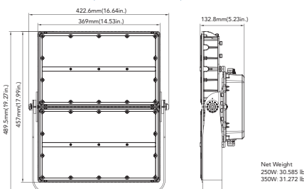
250W/350W(Trunnion Mount)
