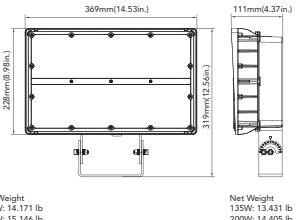
135W&200W(Yoke Mount)
