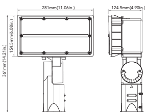
250W/350W(Trunnion Mount)
