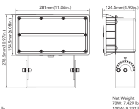
70W&100W(Yoke Mount)
