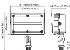
70W&100W(Slipfitter Mount)
