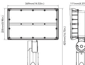
135W&200W(Slipfitter Mount)
