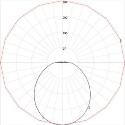
Maximum Candela = 389.08 Located At Horizontal Angle = 225, Vertical Angle = 1 # 1 - Vertical Plane Through Horizontal Angles (225 - 45) (Through Max. Cd.) # 2 - Vertical Plane Through Horizontal Angles (0 - 180) # 3 - Horizontal Cone Through Vertical Angle (1) (Through Max. Cd.)
